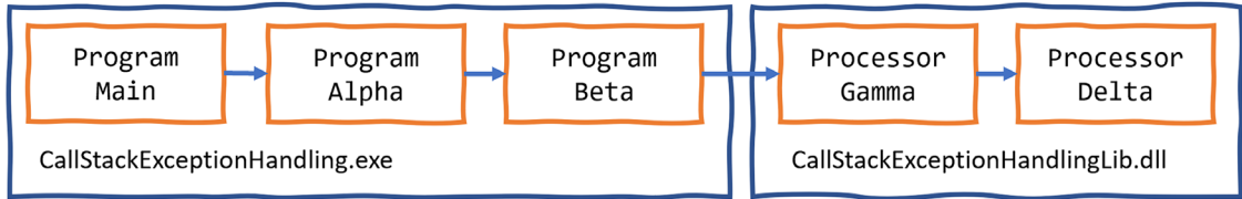
Figure 4.10: A chain of method calls that create a call stack
