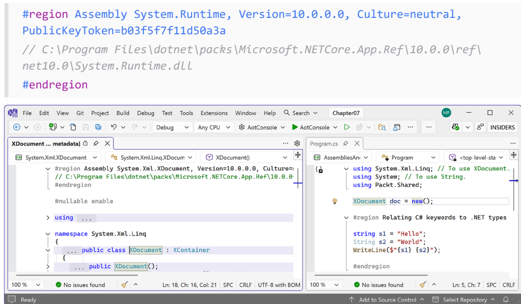
Figure 7.1: Assembly and namespace that contains the XDocument type
