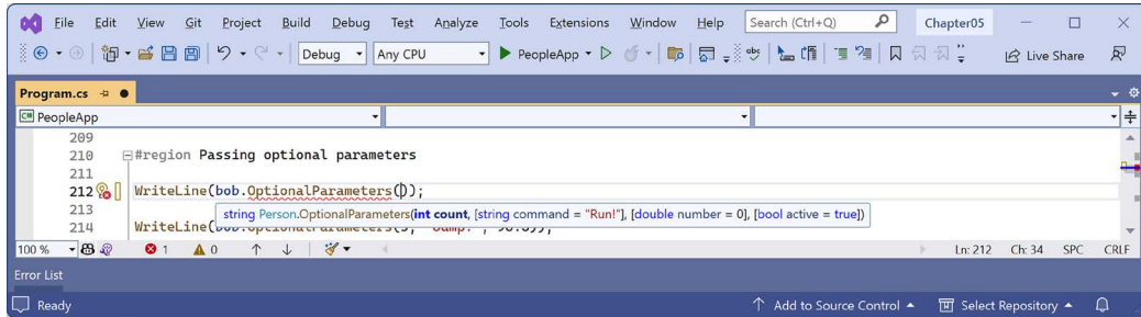
Figure 5.4: IntelliSense showing the required and optional parameters as you type code
