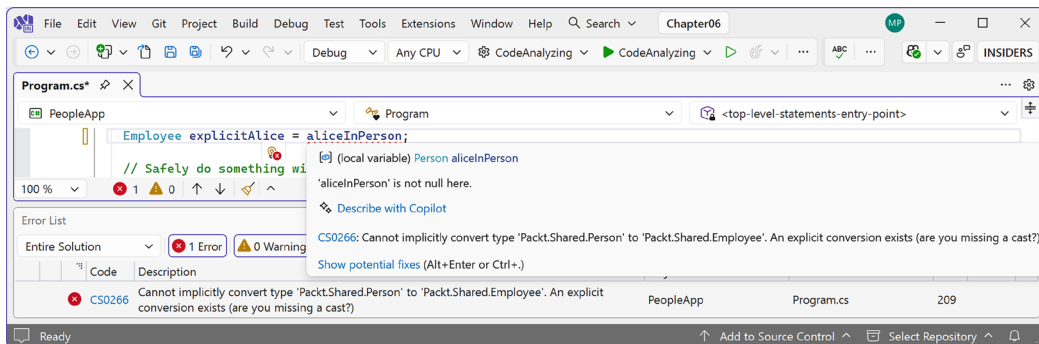
Figure 6.4: A missing explicit cast compile error
