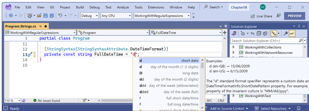
Figure 8.2: IntelliSense activated due to the StringSyntax attribute
