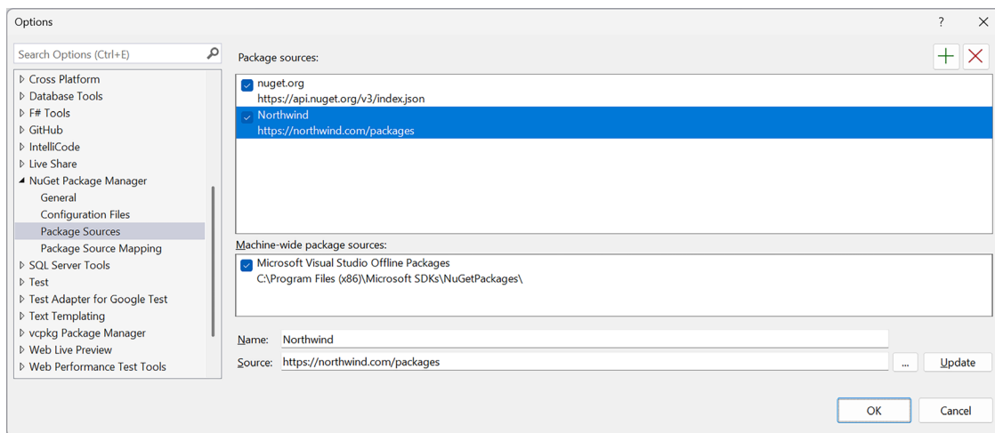
Figure 12.3: Visual Studio with two NuGet package sources configured
