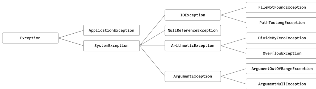
Figure 11.4: A partial exception inheritance hierarchy
