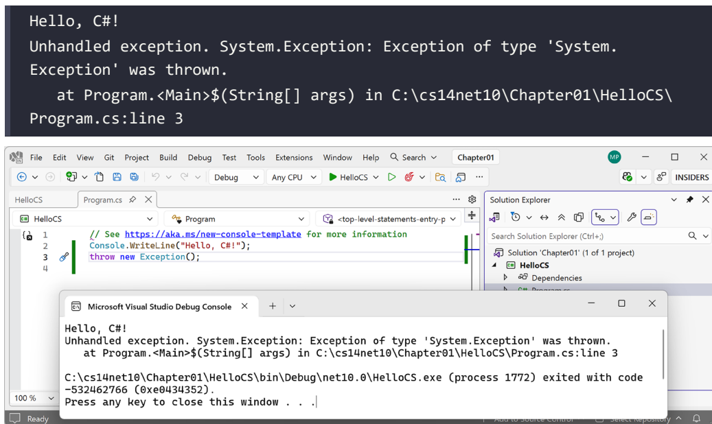
Figure 1.9: Throwing an exception to reveal the hidden Program.<Main>$ method
