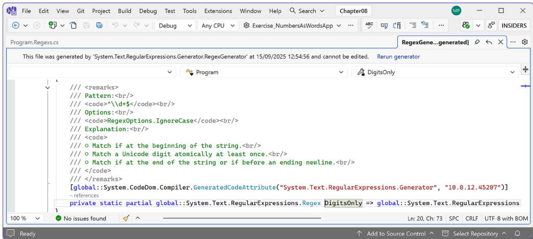
Figure 8.5: The auto-generated source code for the regular expression
