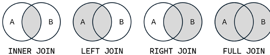
Figure 11.8: Types of join in SQL
