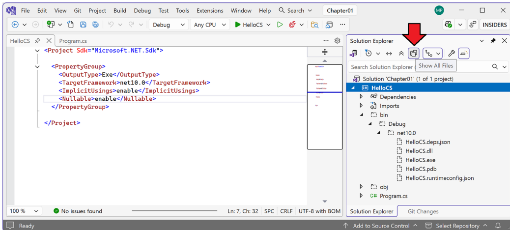
Figure 1.8: Showing the compiler-generated folders and files
