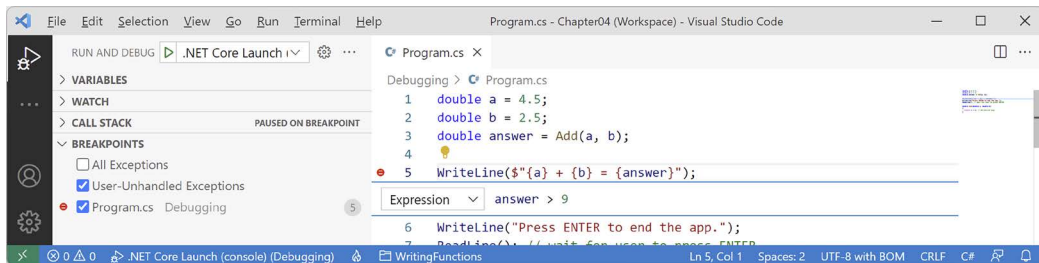
Figure 4.6: Customizing a breakpoint with an expression using VS Code
