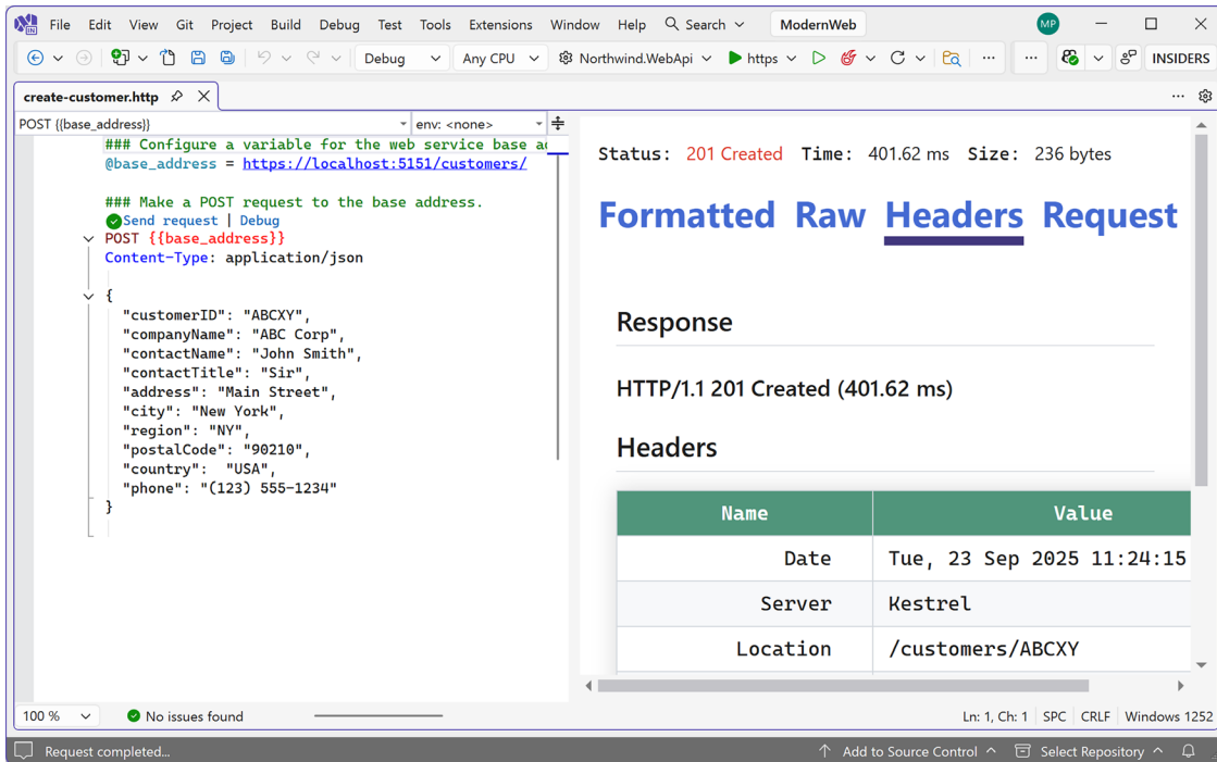
Figure 15.4: Adding a new customer by POSTing to the web service
