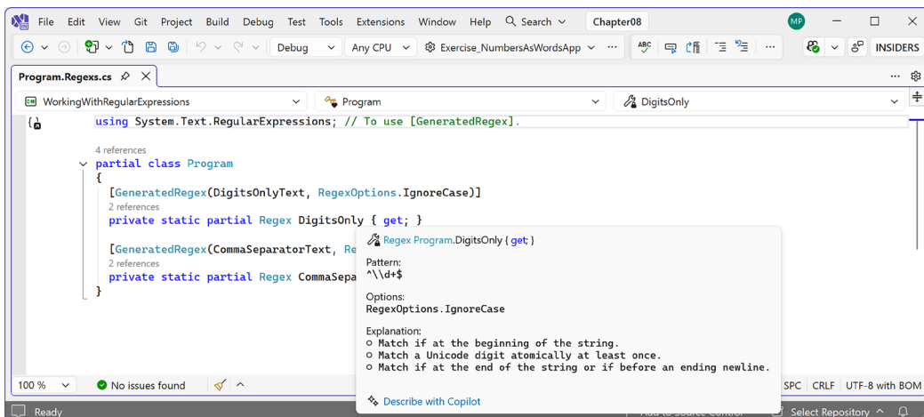
Figure 8.4: Tooltip for a partial method shows a description of the regular expression
