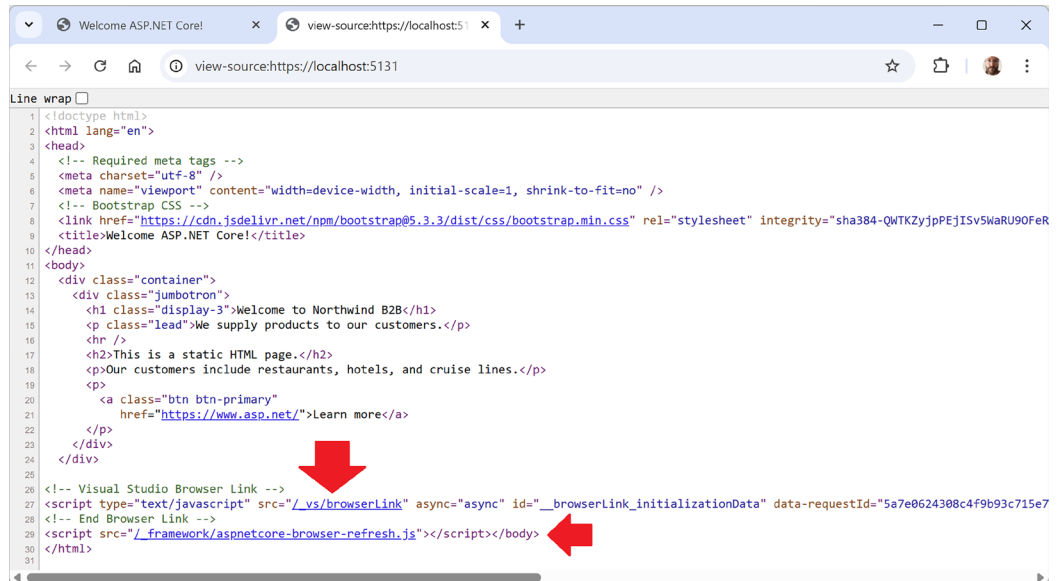
Figure 13.4: Visual Studio dynamically injects scripts to enable features like Browser Link and CSS Hot Reload
