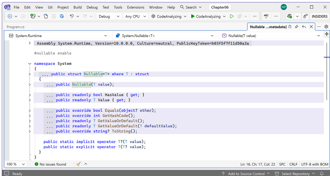
Figure 6.1: Revealing Nullable<T> members
