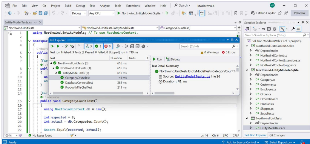
Figure 12.5: Three successful unit tests ran
