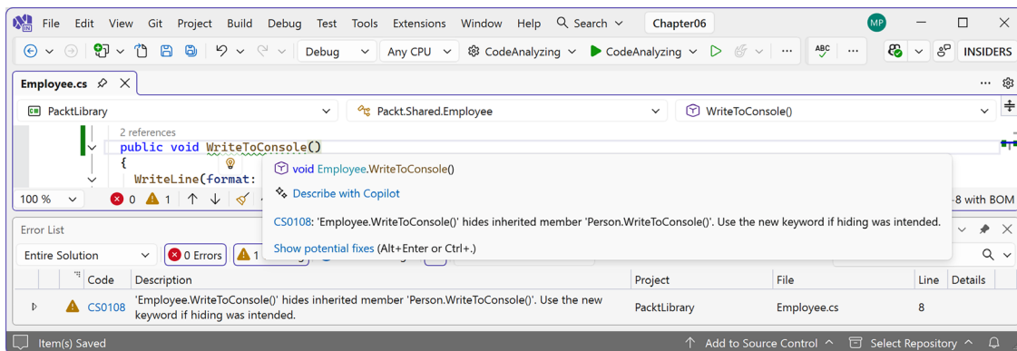
Figure 6.3: Hidden method warning
