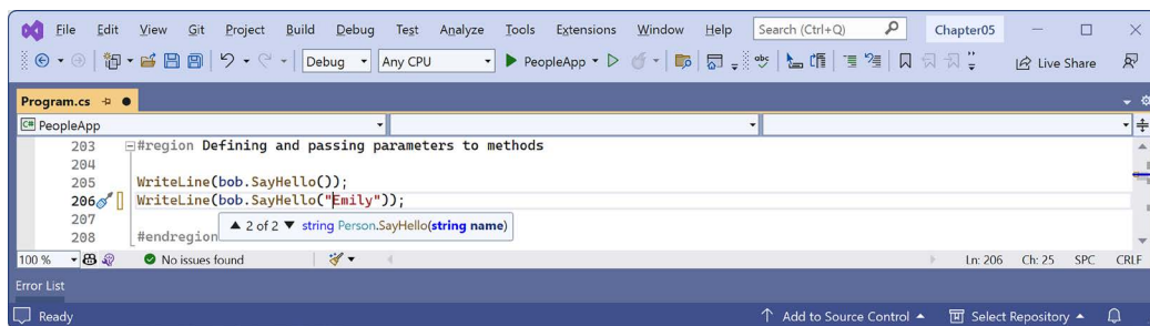
Figure 5.3: An IntelliSense tooltip for an overloaded method
